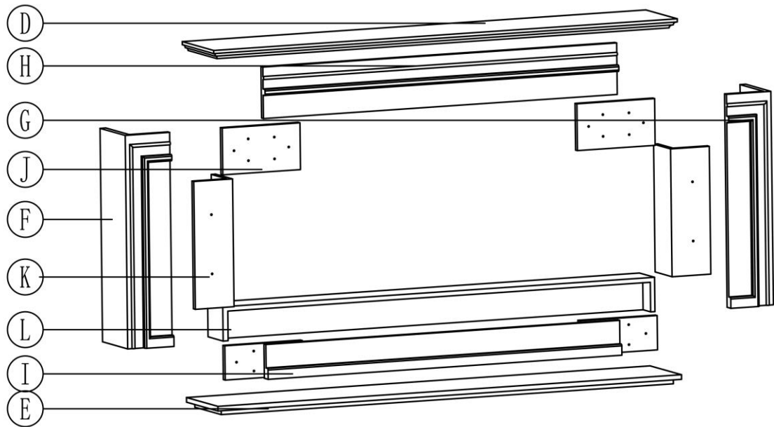
Exploded view of all cabinet pieces
